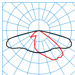
LIQ 70N-AB7L-LR/7500-722 8G1 ET (CLO initial value) TX778339 ■ C0 - C180 ■ C90 - C270 DIN 5040: A30 UTE: 1,00 E DLOR: 100 % ULOR: 0 % CEN Flux Code: 39 76 98 100 100
