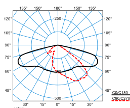
LIQ 70N-AB7L-LR/7500-722 8G1 ET (CLO initial value) TX778339
