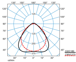
ELINE PW60 830 L150 1 20
