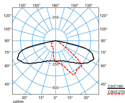
LIQ 50N-AB2L-LRA/22/26/32-722 4G1 ETDD (CLO end value)
