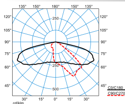
LIQ 50N-AB2L-LRA/22/26/32-722 4G1 ETDD (CLO initial value)
