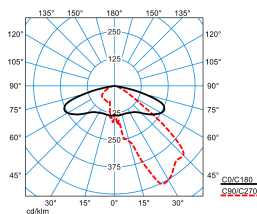
Publisca P1-AB2L/2900-730 4G1S ETDD (CLO end value) TX300792 DIN 5040: A30 UTE: 1,00 G DLOR: 100 % ULOR: 0 % CEN Flux Code: 35 73 97 100 100
