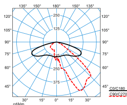
Publisca P1-AB2L/2900-730 4G1S ETDD (CLO initial value) TX301653 DIN 5040: A30 UTE: 1,00 G DLOR: 100 % ULOR: 0 % CEN Flux Code: 35 73 97 100 100
