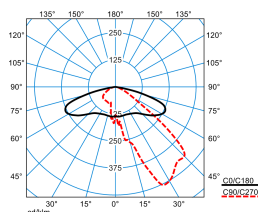
Publisca P1-AB2L/2900-730 4G1S ETDD (CLO initial value)
