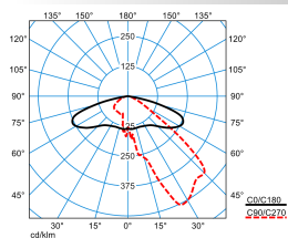
Publisca P1-AB2L/2900-730 4G1S ETDD (CLO initial value)
