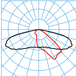
LIQ 50N-AB2L-LR/4200-740 4G1 ET (CLO end value) TX777875 ■ C0 - C180 ■ C90 - C270 DIN 5040: A30 UTE: 1,00 G DLOR: 100 % ULOR: 0 % CEN Flux Code: 34 71 96 100 100 0 0 0 0
