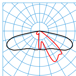
Publisca P2-AB2L/1350-740 2G1S ETDD (CLO initial value) TX301009 ■ C0 - C180 ■ C90 - C270 DIN 5040: A30 UTE: 1,00 G DLOR: 100 % ULOR: 0 % CEN Flux Code: 34 70 96 100 100
