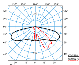
Publisca P2-AB2L/1200-730 2G1S ETDD (CLO initial value) TX300988 DIN 5040: A30 UTE: 1,00 G DLOR: 100 % ULOR: 0 % CEN Flux Code: 34 70 96 100 100
