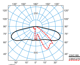
Publisca P2-AB2L/1200-730 2G1S ETDD (CLO end value) TX300420 DIN 5040: A30 UTE: 1,00 G DLOR: 100 % ULOR: 0 % CEN Flux Code: 34 70 96 100 100
