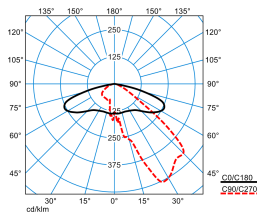
Publisca P1-AB2L/3200-740 4G1S ETDD (CLO end value) TX300239 DIN 5040: A30 UTE: 1,00 G DLOR: 100 % ULOR: 0 % CEN Flux Code: 35 73 97 100 100
