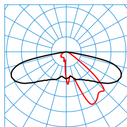
Publisca P2-AB2L/2000-740 3G1S ETDD (CLO initial value) TX301083 ■ C0 - C180 ■ C90 - C270 DIN 5040: A30 UTE: 1,00 l DLOR: 100 % ULOR: 0 % CEN Flux Code: 34 71 96 100 100
