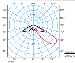
LnPlus 60-AM19L/26000-730 24G1 ETDD (CLO initial value)
