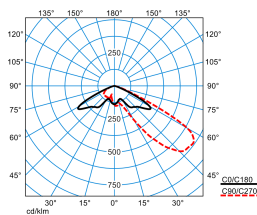
LnPlus 60-AM19L/26000-730 24G1 ETDD (CLO end value)
