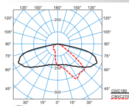
LIQ 50N-AB2L-LRA/51/56/62-722 6G1 ETDD (CLO initial value)
