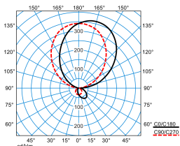
Sanesca W2 LED5000-830 01
