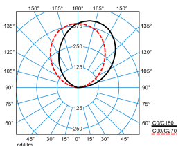
Sanesca W2 LED5000-830 01 (room light)
