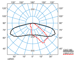
LIQ 50N-AB2L-LR/6800-727 6G1 ET (CLO initial value)
