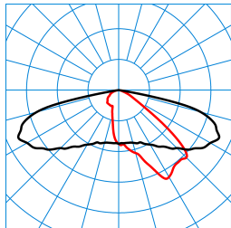
LIQ 50N-AB2L-LR/1200-722 2G1 ET (CLO initial value) TX777308 ■ C0 - C180 ■ C90 - C270 DIN 5040: A30 UTE: 1,00 G DLOR: 100 % ULOR: 0 % CEN Flux Code: 34 71 96 100 100 0 0 0 0
