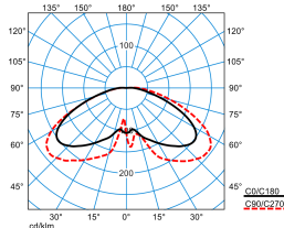
Publisca P1W-RBT-LR/2600-740 3G1S TX053574 DIN 5040: A20 UTE: 0.99 l + 0.01 T DLOR: 99 % ULOR: 1 % CEN Flux Code: 26 63 91 99 100 0 0 0 1
