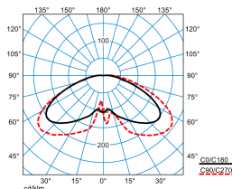
Publisca P1W-RBT-LR/2600-740 3G1S ET (CLO end value) TX300324 DIN 5040: A20 UTE: 0.99 l + 0.01 T DLOR: 99 % ULOR: 1 % CEN Flux Code: 26 63 91 99 100 0 0 0 1
