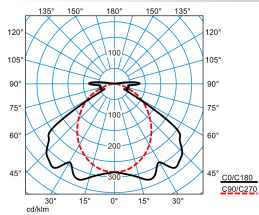
Nextrema G3 B 4000-840 ET +HFS TX770194
