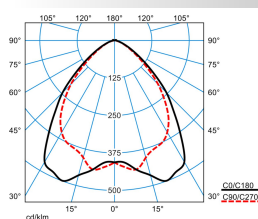
ELINE LW40-110 ML 830 L150 0 20
