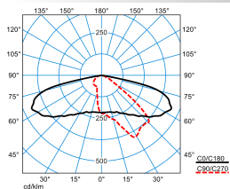
LIQ 50N-AB2L-LR/220/260/320-730 4G1 ET (CLO initial value)
