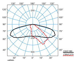
LIQ 50N-AB2L-LR/220/260/320-730 4G1 ET (CLO end value)
