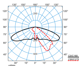
Publisca P2-AB2L/3800-740 6G1S ETDD (CLO initial value)
