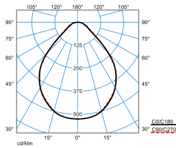
Belviso C1 625 CDP LED3900ww ETDD 01 TX773206
