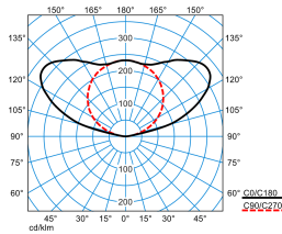
E-Line PRO 78HE I-UW 20-830ETDD L75 05 05
