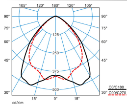
ELINE LW180 830 L225 1 20
