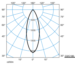
Amatris RC1 SRRFL 8-9MC ETD-PD 05 + HC-19 05 (stage 2)
