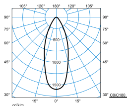
Amatris RC1 SRRFL 8-9MC ETD-PD 05 + PC IP54 (stage 1)
