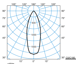
Amatris RC1 SRRFL 8-9MC ET-PD 05 (stage 2)
