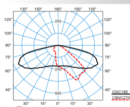
LIQ 50N-AB2L-LRA/135/165/20-730 2G1 ETDD (CLO initial value)
