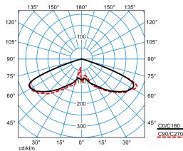
Publisca P1-RB6L-LRA/2400-730 3G1S
