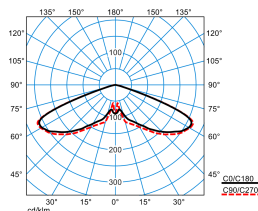
Publisca P2-RB6L/3200-730 4G1S ETDD (CLO end value)
