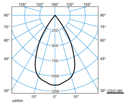
E-Line PRO 78 BV G2 RF-VFL 35-BF M54 ETBLE 01 01
