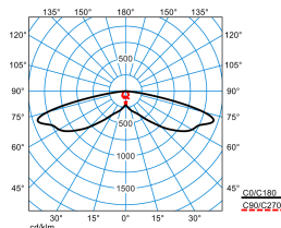
Publisca P2-SB3L/800-740 2G1S ETDD (CLO initial value)
