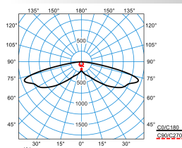
Publisca P2-SB3L/800-740 2G1S ETDD (CLO end value)
