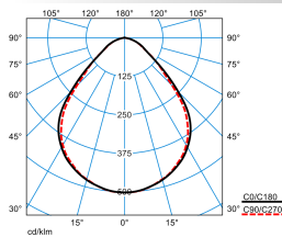
Opendo D2-L PW19 42-8TW ETBLE +CAS-S 01 (DWW) TX874507
