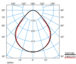
Opendo D2-L PW19 42-8TW ETBLE +CAS-S 01 (DSU)
