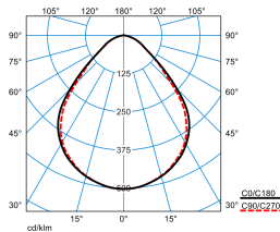
Opendo D2-L PW19 42-8TW ETBLE +CAS-S 01 (DSU) TX874506
