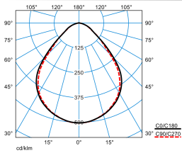
Opendo D2-L PW19 42-8TW ETBLE +CAS-S 01 (DWW)
