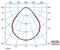
Opendo D2-L PW19 42-8TW ETBLE +CAS-S 01 (DCW)
